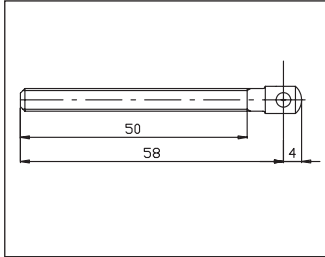
Chain tie-rod for special installation (for example wood or PVC window frame) part No. 81222C
