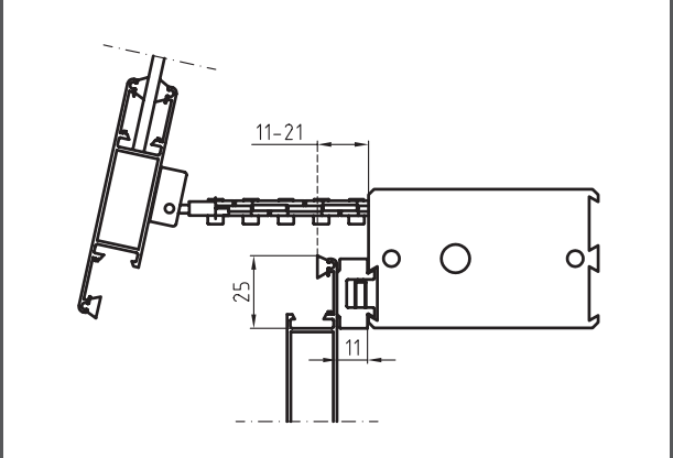
On the frame with the sliding fixing bracket included
